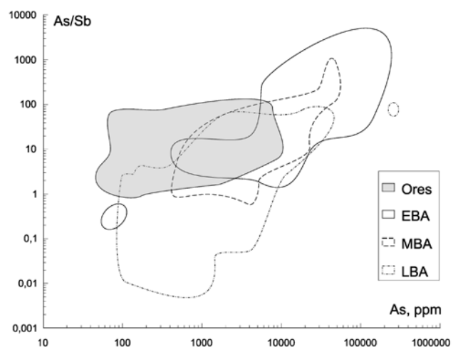
Fig. 7: Plot of As versus As/Sb ratios in Armenian copper ores and copper-based artefacts. Most Early Bronze Age artefacts seem to be enriched in arsenic compared with the copper ores. Also Middle Bronze Age artefacts show some enrichment of arsenic and antimony but it is less pronounced than in the Early Bronze Age. In Late Bronze Age very low As/Sb ratios are generally characteristic for most of the analysed artefacts.
