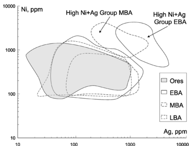
Fig. 6: Plot of Ag versus Ni for Armenian copper ores and copper based artefacts. Some Early and Middle Bronze Age artefacts exhibit high concentrations of nickel and silver. In the Late Bronze Age the High Ni and Ag group disappears.
